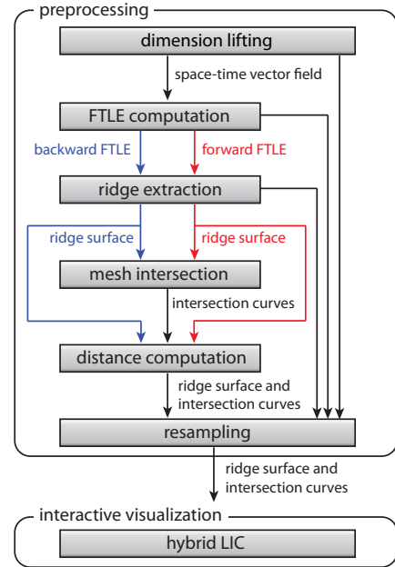
Figure 4: Overview of our technique, accompanied by the data that are passed between the stages of the pipeline.
