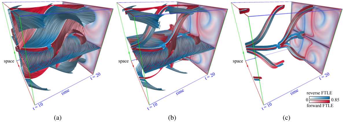
Figure 7: Quad-Gyre example. The advection time for forward and reverse FTLE is T = 7.5s . (a) Full visualization of forward and reverse LCS. A lower FTLE threshold of 0.4 is used. (b) Visualization restricted to complementary FTLE bands. Minor artifacts appear due to aliasing effects of forward and reverse FTLE. The minimum complementary FTLE value is 0.19. (c) Restriction to distance-based LCS intersection bands reveals the topological space-time skeleton.
