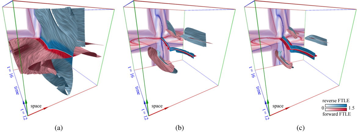
Figure 3: Building blocks for space-time LCS visualization, shown with the example from Sec. 5.1. Advection time for forward and reverse FTLE is T = 4s . (a) Space-time LIC qualitatively visualizes LCS dynamics: hyperbolic behavior is apparent. In addition, hyperbolicity is encoded by color saturation. A minimum FTLE value of 0.5 is used. (b) Intersection bands by clipping with complementary FTLE reduce occlusion but still provide context and convey structure of reverse FTLE. The minimum complementary FTLE value is 0.41. (c) Intersection bands by clipping with distance to intersection curves further reduces occlusion and provides the topological skeleton.
