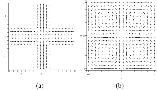
Figure 5: (a) Gyre Saddle example at t = 0 . (b) Quad Gyre example at t = 0 .
