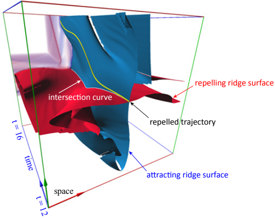
Figure 2: Space-time ridge surfaces in forward (red) and reverse (blue) finite-time Lyapunov exponent together with cross section at final time step (colored). The space-time intersection curve in the center (white) represents a hyperbolic trajectory. Traditional integration of the hyperbolic trajectory from the initial intersection is difficult due to exponential growth of error (yellow curve).
